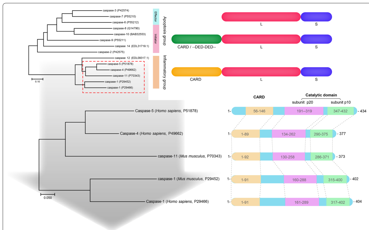
Fig. 3 Caspase family homology comparison (Source: https://www.ncbi.nlm.nih.gov/ ). A phylogenetic tree was constructed by the N-J method to compare the homology among members of the Caspase family. CARD, Caspase activation and recruitment domains; L + S, catalytic domain, L as p20 subunit and S as p10 subunit. Protein domains were predicted by interpro ( www.ebi.ac.uk/interpro/scan )
